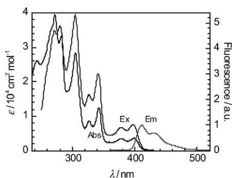
Figure 7. Absorption, fluorescence excitation, and fluorescence emission spectra of 9 in chloroform.
