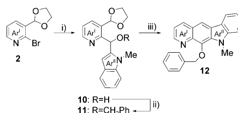
Scheme 3. Synthesis of pyridocarbazole derivative 12 . Conditions: i) n BuLi, -78^{\circ}\text{C} , 10 min, THF followed by N -methylindole-2-carboxaldehyde, -78 \rightarrow 0^{\circ}\text{C} , 59%; ii) NaH, RT, 30 min, THF followed by \text{C}_6\text{H}_5\text{CH}_2\text{Br} (1.5 equiv), KI (5%), 18 h, RT, 99%; iii) 1 N HCl, acetone, 3 d, RT, 34%.
