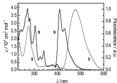
Figure 5. UV/Vis absorption (left) and fluorescence emission spectra (right) of 5 and 9 in chloroform.
