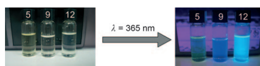
Figure 4. Fluorescence of compounds 5 , 9 , and 12 in solution (CDCl 3 ) before and after UV exposure.
