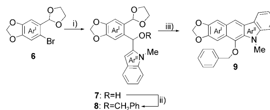
Scheme 2. Synthesis of benzocarbazole derivative 9 . Conditions: i) n BuLi, -78^{\circ}\text{C} , 10 min, THF followed by N -methylindole-2-carboxaldehyde, -78 \rightarrow 0^{\circ}\text{C} , 66%; ii) NaH, RT, 30 min, THF followed by \text{C}_6\text{H}_5\text{CH}_2\text{Br} (1.5 equiv), KI (5%), 18 h, RT, 79%; iii) 1 N HCl, acetone, 30 min, RT, 99%.
