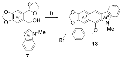
Scheme 4. Synthesis of benzocarbazole derivative 13 . Conditions: i) NaH, RT, 30 min, THF followed by \alpha,\alpha' -dibromo- p -xylene, 18 h, RT, 39 %.
