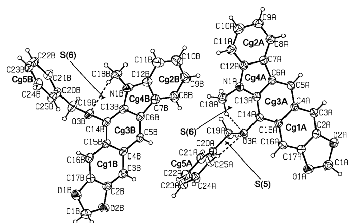
Figure 1. Views of molecules A (right) and B (left) in the crystal structure of 9 , showing the atom numbering schemes. Displacement ellipsoids are drawn at the 30% probability level and hydrogen atoms are shown as small spheres of arbitrary radius. Cg denotes the centroid of the aromatic rings. The dashed lines depict intramolecular hydrogen bonds that generate the S(5) and S(6) graph-set motifs.
