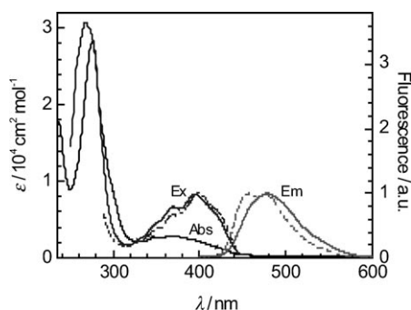
Figure 6. Absorption, fluorescence excitation, and fluorescence emission spectra of 5 in chloroform (solid lines) and toluene (dotted lines).
