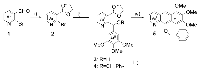
Scheme 1. Synthesis of benzoquinoline derivative 5 . Conditions: i) HOCH 2 CH 2 OH/4-MeC 6 H 4 SO 3 H (cat.), benzene, reflux, 4 h, 94 %; ii) n -BuLi, –78 °C, 10 min, THF followed by 3,4,5-C 6 H 2 (OMe) 3 CHO, –78 → 0 °C, 69 %; iii) NaH, RT, 30 min, THF followed by C 6 H 5 CH 2 Br (1.5 equiv), KI (5 %), 18 h, RT, 83 %; iv) 1 N HCl, MeOH, 5 d, RT, 53 %.
