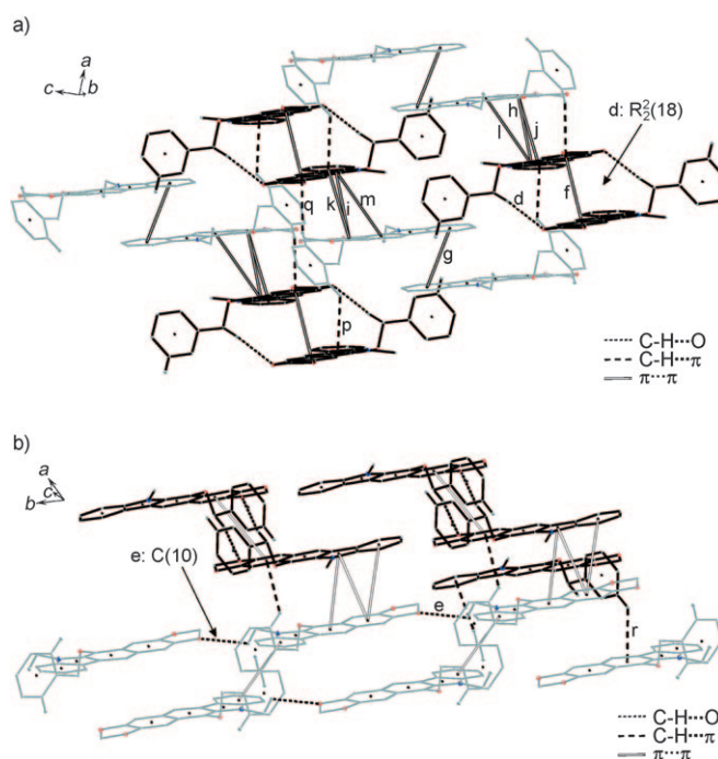
Figure 2. a, b) Parts of the crystal structure of 9 showing the intermolecular C–H \cdots O hydrogen bonds that form the R_2^2(18) graph-set dimers (motif d), and the C(10) chains (motif e). Molecules A and B are depicted by black and grey, respectively. Other interactions: f) Cg1A \cdots Cg1A (iii) ; g) Cg2B \cdots Cg2B (iv) ; h) Cg4A \cdots Cg1B (iii) ; i) Cg1B \cdots Cg4A (iii) ; j) Cg2A \cdots Cg1B (iii) ; k) Cg1B \cdots Cg2A (iii) ; l) Cg4A \cdots Cg3B (iii) ; m) Cg3B \cdots Cg4A (iii) ; p) C21B–H21B \cdots Cg2A (iv) (C21B–H21B = 0.93 , H21B \cdots Cg2A = 2.85 , C21B \cdots Cg2A = 3.565(3) Å; C21B–H21B–Cg2A = 135^\circ ); q) C25B–H25B \cdots Cg1A (iii) (C25B–H25B = 0.93 , H25B \cdots Cg1A = 2.89 , C25B \cdots Cg1A = 3.586(3) Å; C25B–H25B–Cg1A = 133^\circ ); r) C22A–H22A \cdots Cg3B (v) (C22A–H22A = 0.93 , H22A \cdots Cg3B = 2.82 , C22A \cdots Cg3B = 3.582(3) Å; C22A–H22A–Cg3B = 140^\circ ). Symmetry codes: (i) -x, -y, -z ; (iii) 1-x, -y, 1-z ; (iv) -x, 1-y, 1-z ; (v) -x, -y, 1-z . The centroids of the aromatic rings (Cg; see Figure 1) are denoted by small black spheres. Distances between the ring centroids lie in the range of 3.835(1) – 4.435(2) Å and interplanar angles lie in the range of 0.00 – 7.34^\circ . Hydrogen atoms not involved in the interactions have been omitted for clarity.
