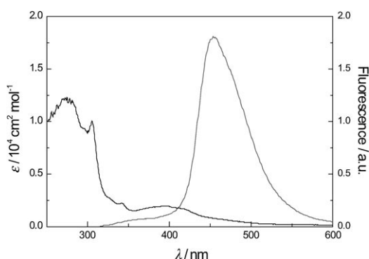
Figure 8. Absorption (left) and fluorescence emission (right) spectra of 12 in chloroform.
