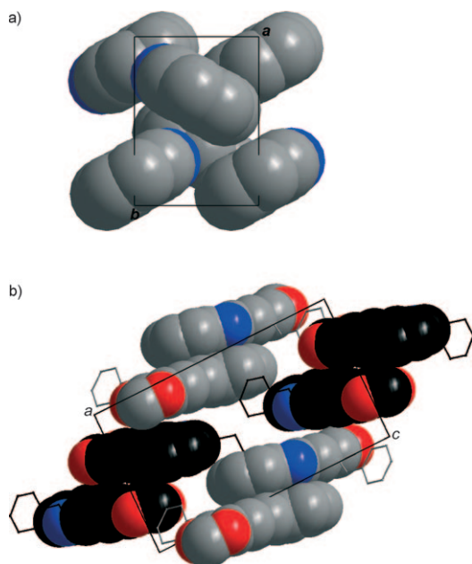
Figure 3. Packing structures of 9 and carbazole in the crystal structures. a) Herringbone packing diagram of carbazole with a space-filling model. b) Columnar stacks of 9 with a space-filling model for planar moiety 1 and a ball-and-stick model for the benzyloxy substituent. All hydrogen atoms have been omitted for clarity.
